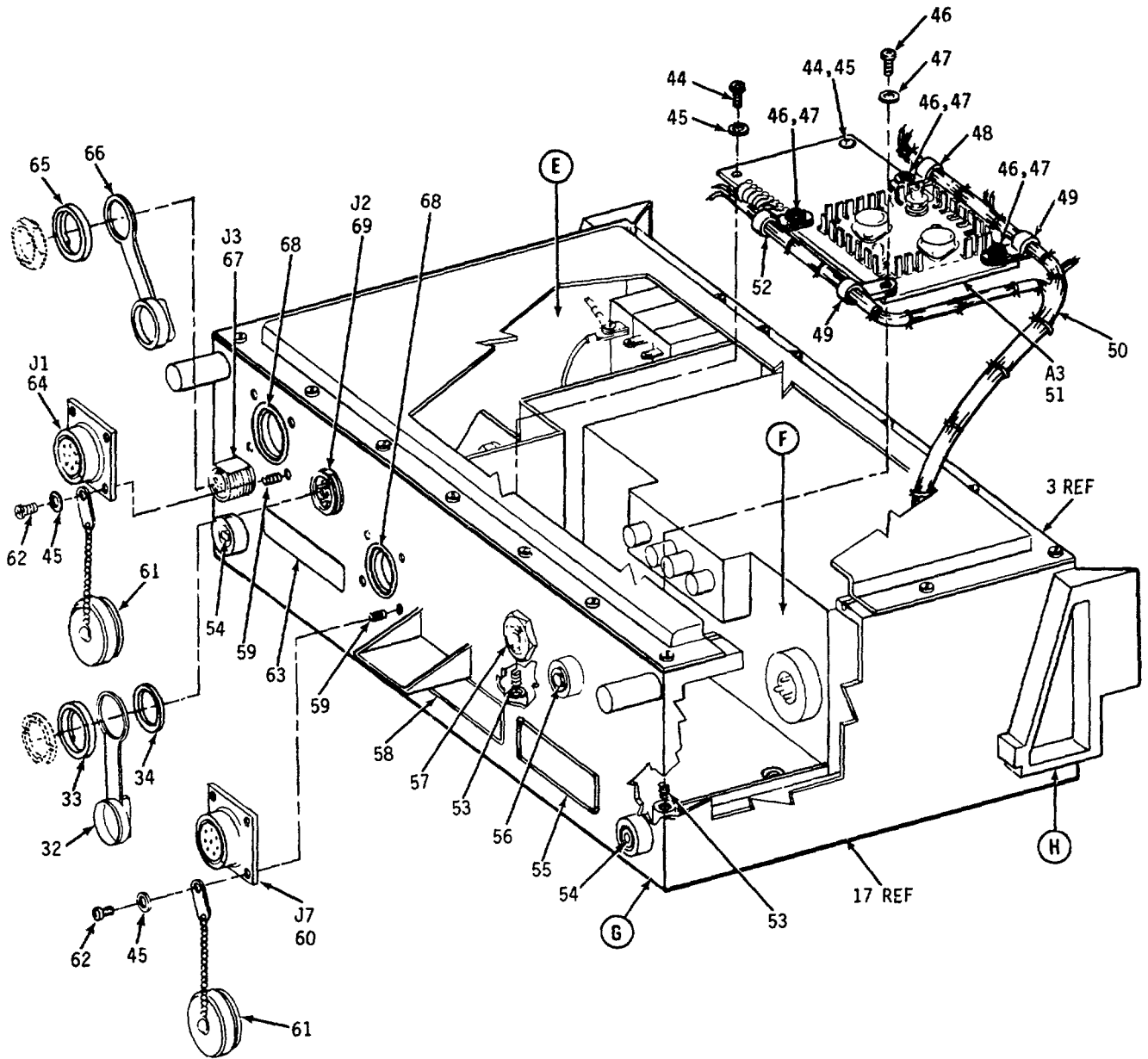
REAR VIEW
