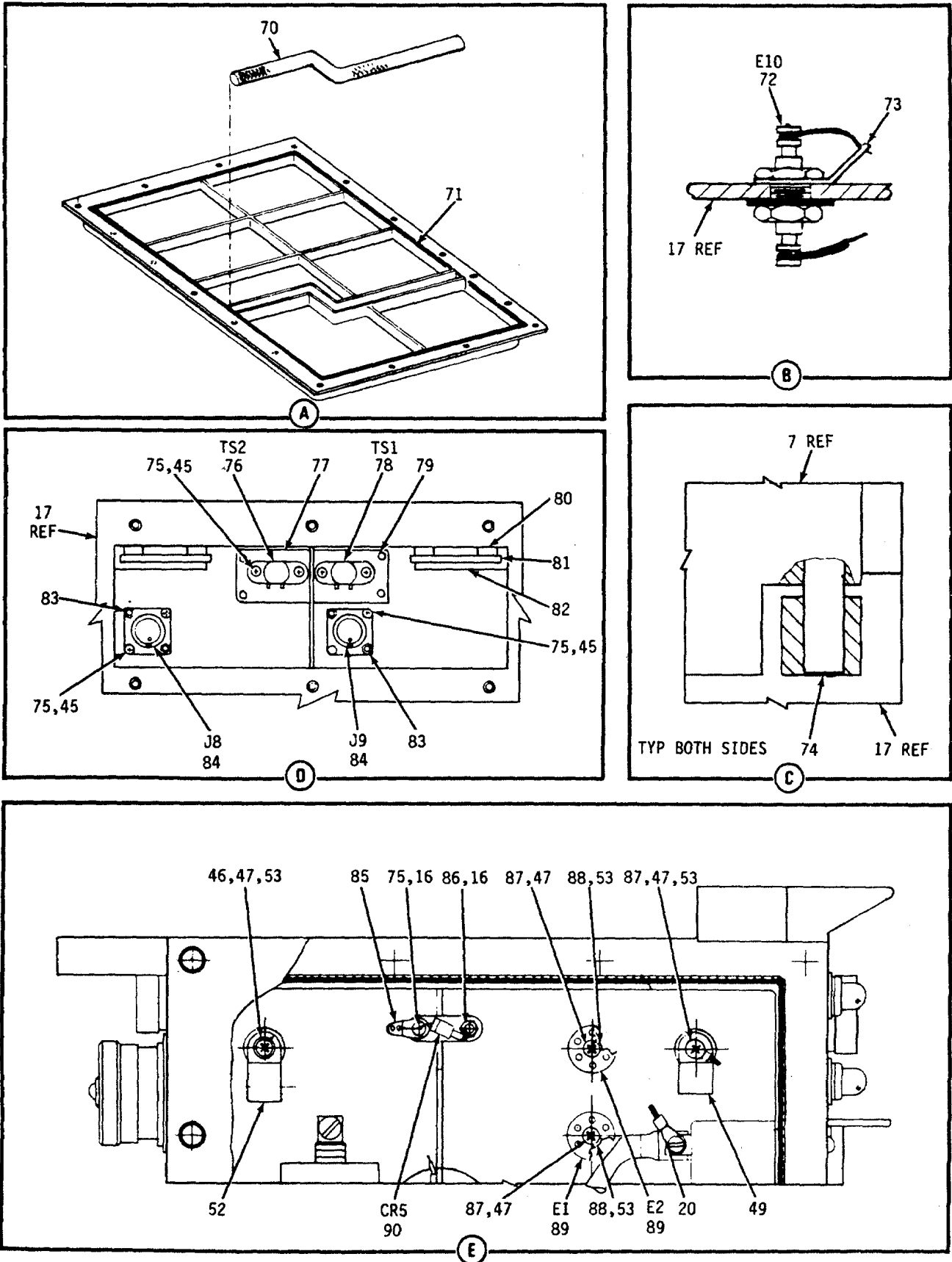
Figure 30. Power Distribution Unit (Sheet 4 of 5)
