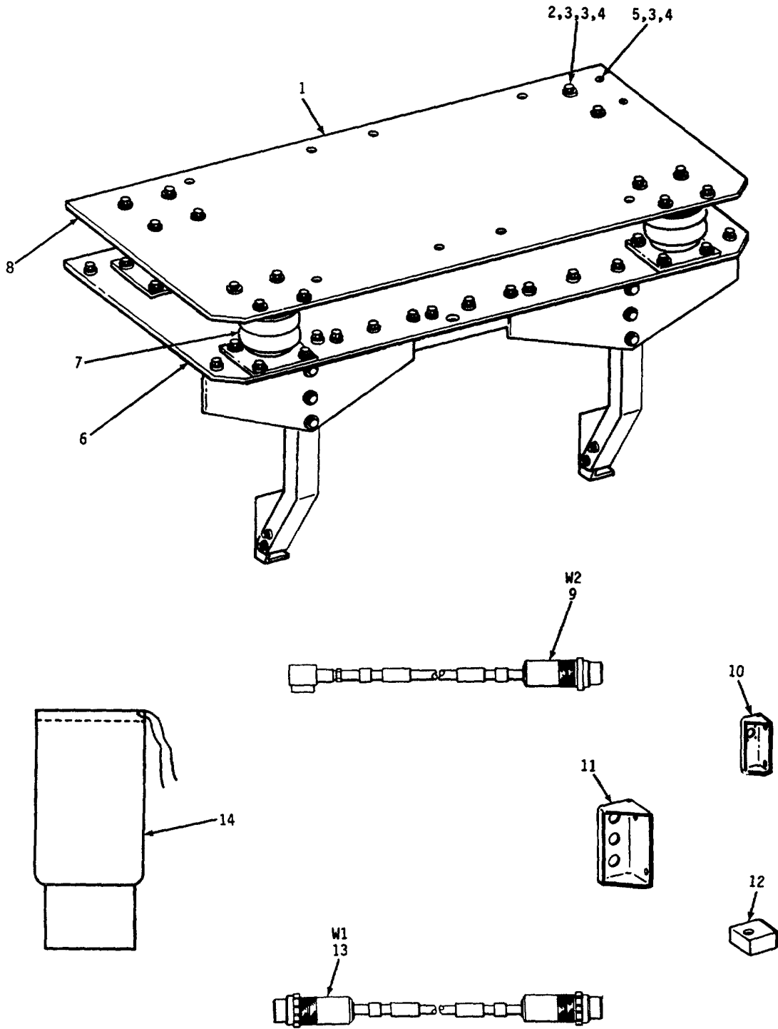
Figure 49. Mounting Kit Assembly MK-1832/GYK-29 (V) (Sheet 1 of 2)
