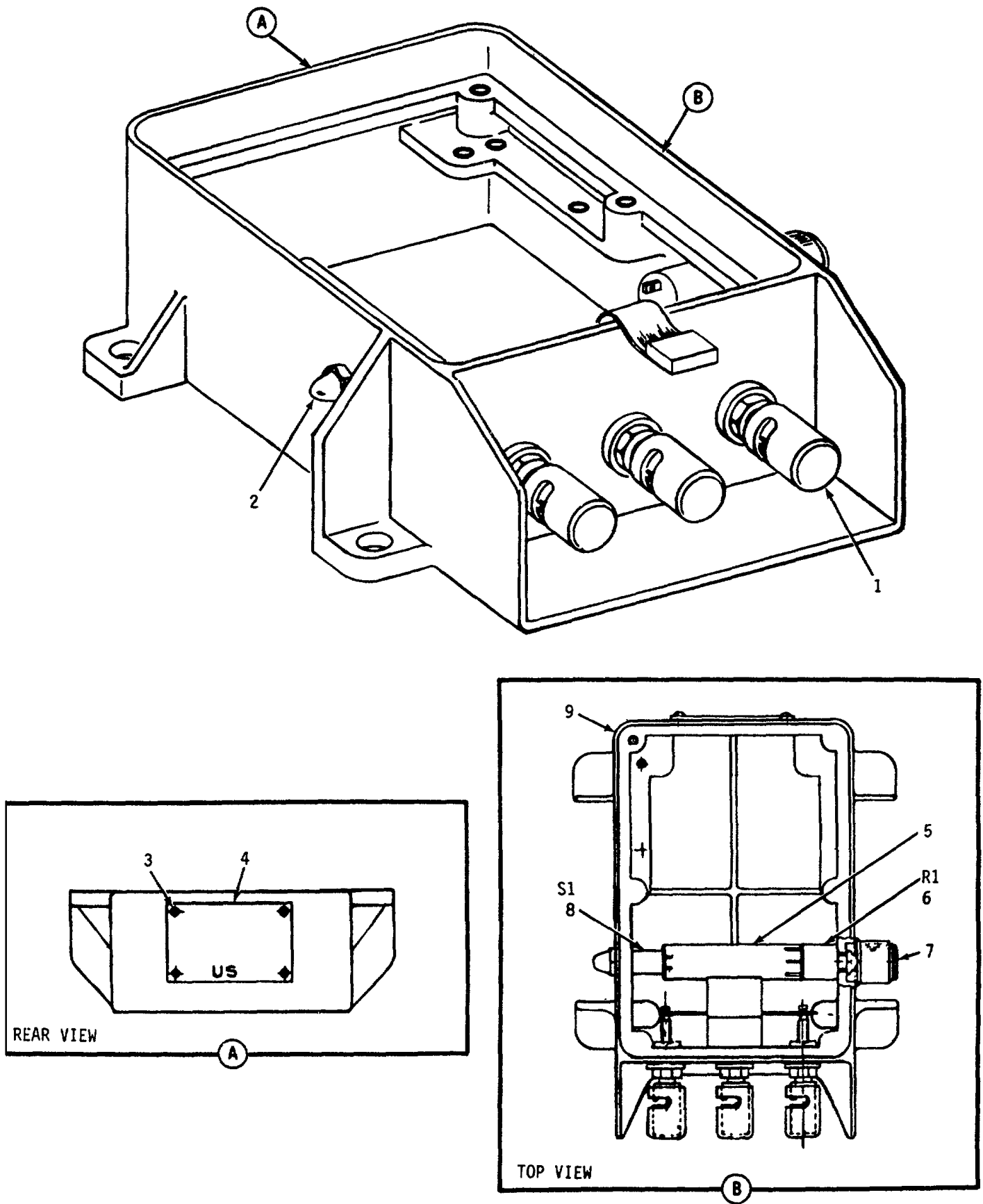
Figure 40. Housing Assembly, GA
