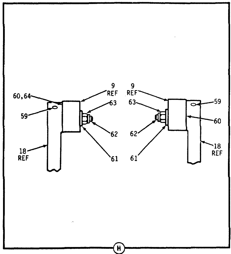
Figure 25. Housing Assembly (Sheet 4 of 6)
