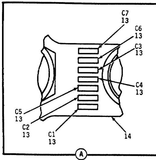
Figure 37. Housing Assembly, SCA
