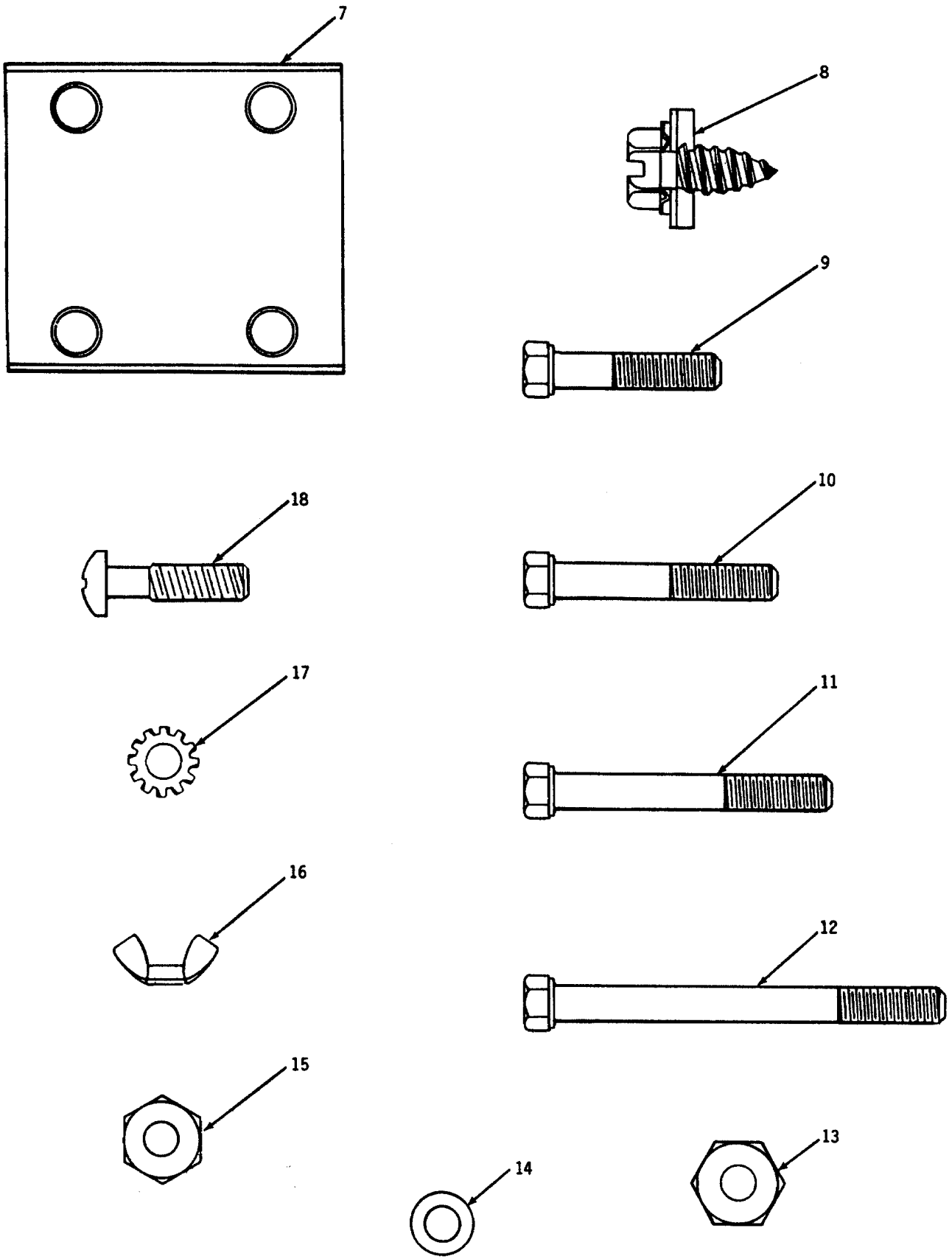
Figure 48. Mounting Kit Assembly MK-1831/GYK-29 (V) (Sheet 2 of 2)
