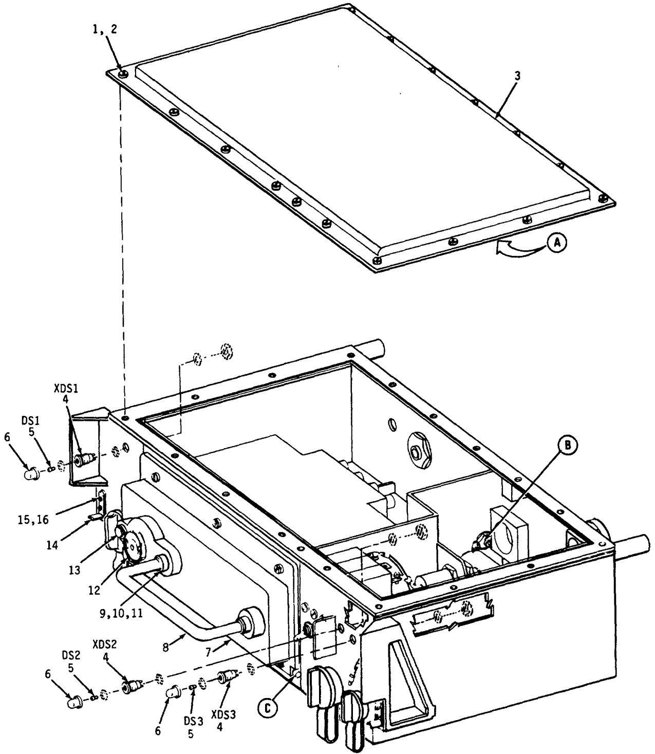
Figure 30. Power Distribution Unit (Sheet 1 of 5)
