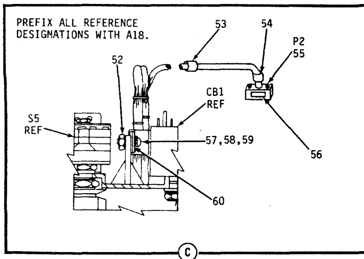
Figure 23. Control Panel Assembly (Sheet 3 of 3)
