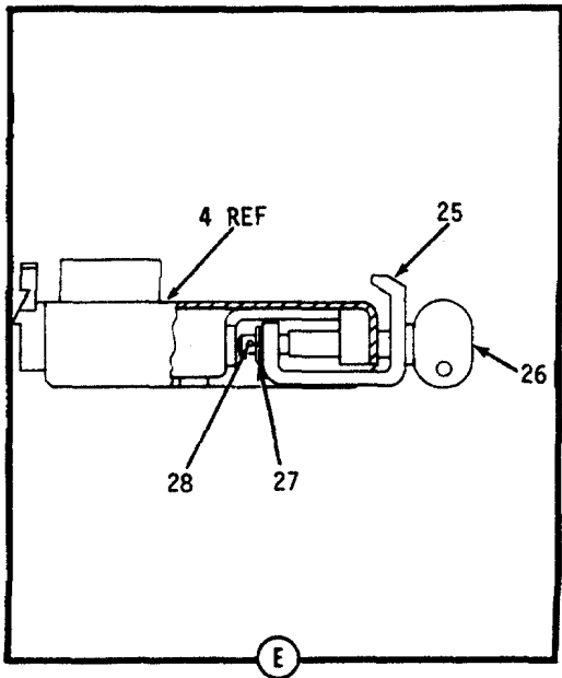
Figure 32. Mounting Base, Computer Gun Direction MT-4938/GYK-29(V) (Sheet 2 of 5)
