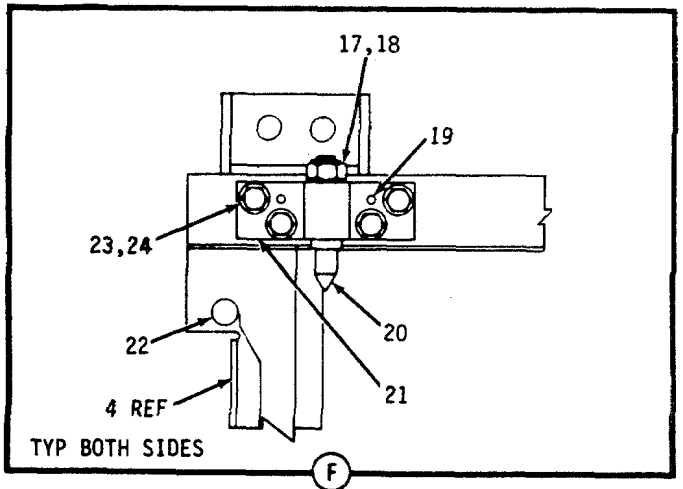
Figure 32. Mounting Base, Computer Gun Direction MT-4938/GYK-29(V) (Sheet 2 of 5)
