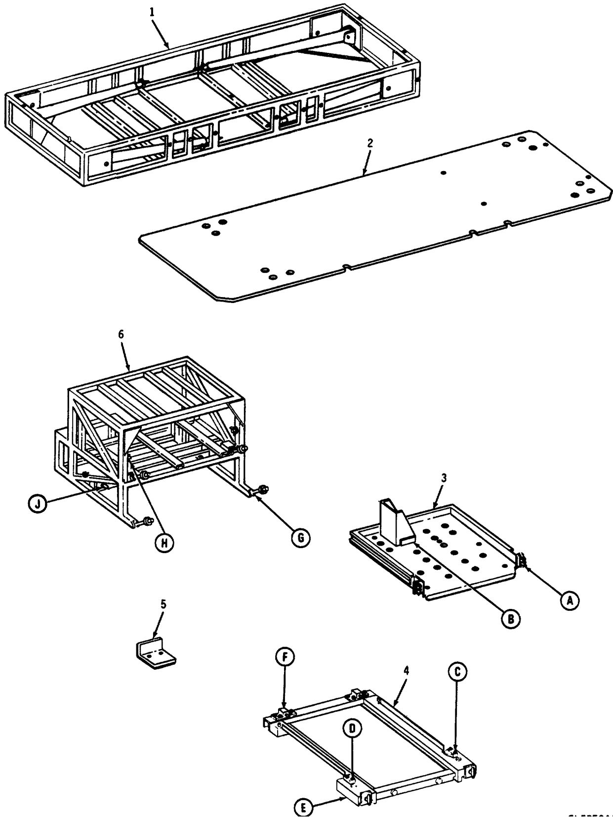
Figure 32. Mounting Base, Computer Gun Direction MT-4938/GYK-29(V) (Sheet 1 of 5)
