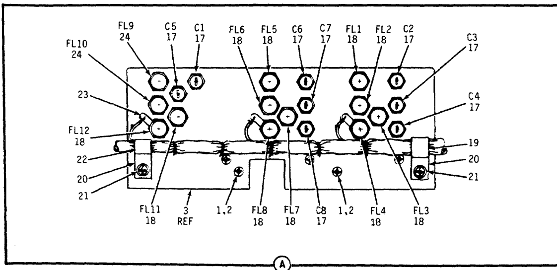
Figure 27. Comm Channel Filter Assembly
