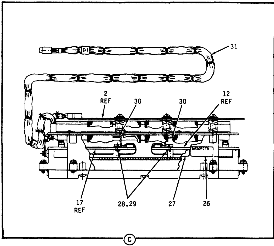
Figure 17. Plasma Panel Assembly (Sheet 2 of 2)
