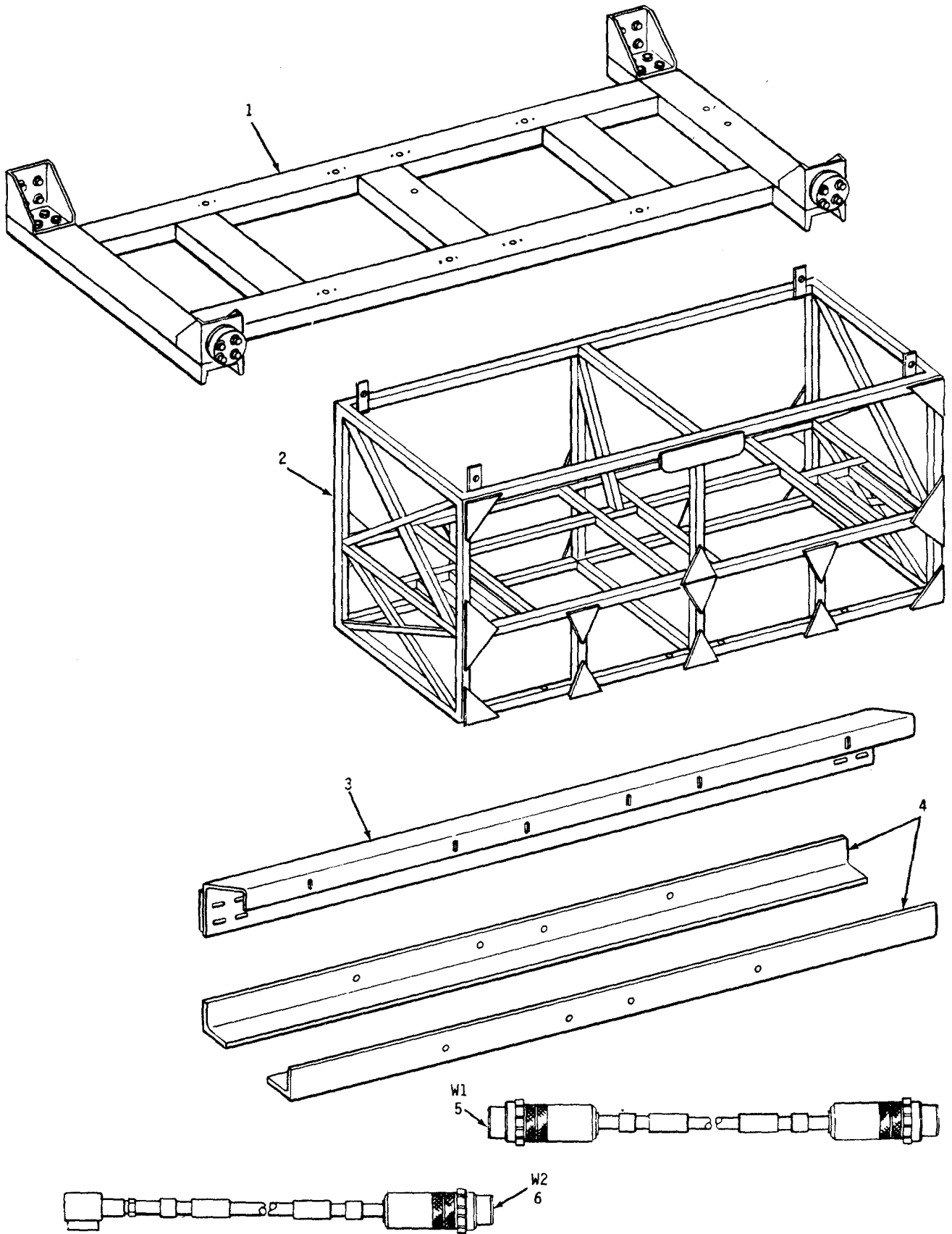
Figure 48. Mounting Kit Assembly MK-1831/GYK-29(V) (Sheet 1 of 2)
