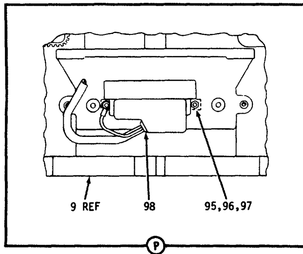
Figure 25. Housing Assembly (Sheet 6 of 6)
