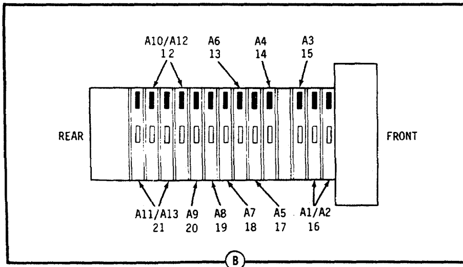
Figure 3. Computer, Gun Direction CP-1317/GYK-29(V) (Sheet 2 of 2)
