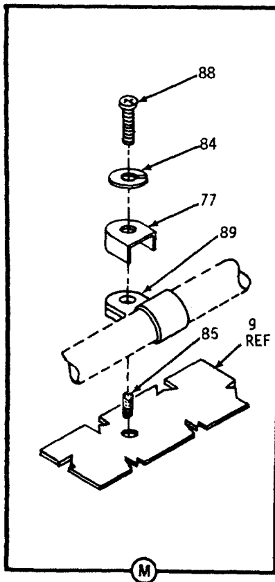
Figure 25. Housing Assembly (Sheet 5 of 6)
