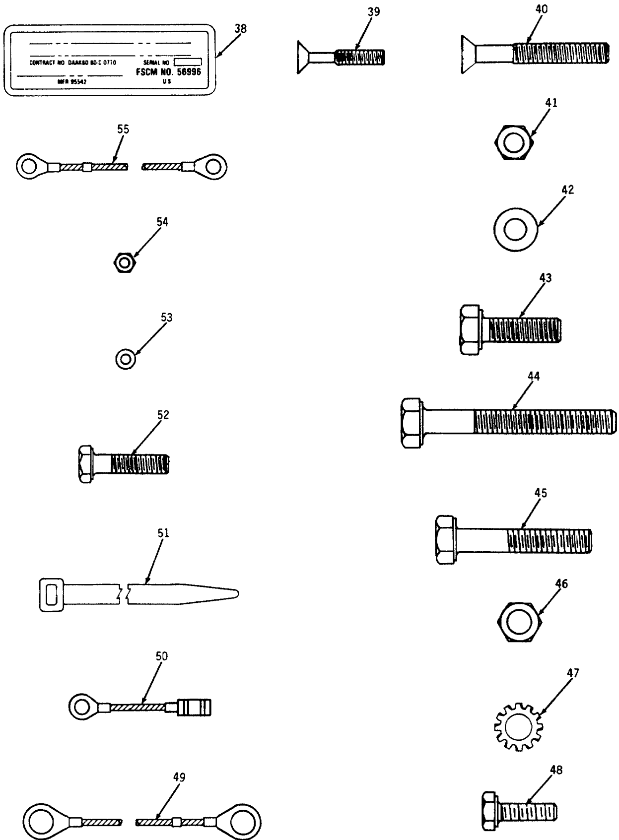
Figure 32. Mounting Base, Computer Gun Direction MT-4938/GYK-29(V) (Sheet 4 of 5)
