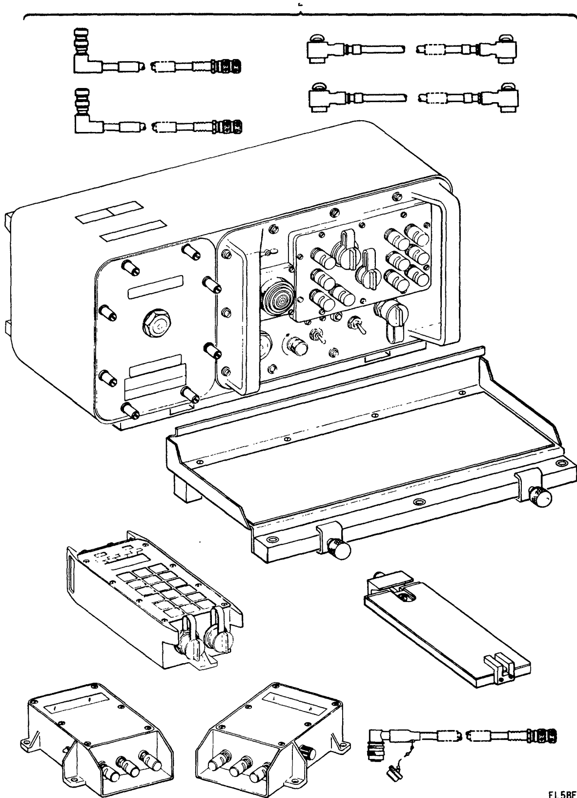
Figure 1. Battery Computer System AN/GYK-29(V) (Sheet 4 of 5).
